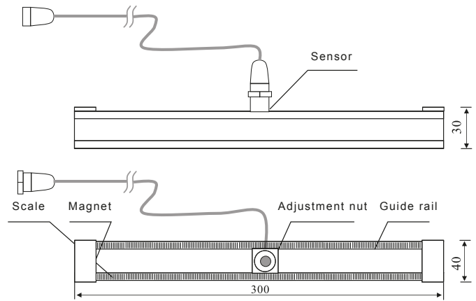
Transducer Dimensions (Unit: mm)
